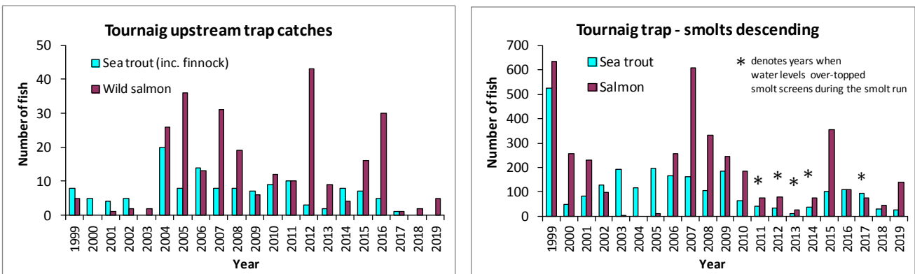
Figure 2.3 Trap catches at Tournai, 1999 to 2019. (left) Upstream trap; (right) downstream trap.
