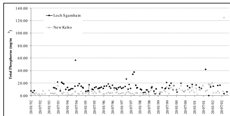
Figure 3.5. Total phosphorus concentrations in the River Carron as measured at the two SEPA monitoring stations.
