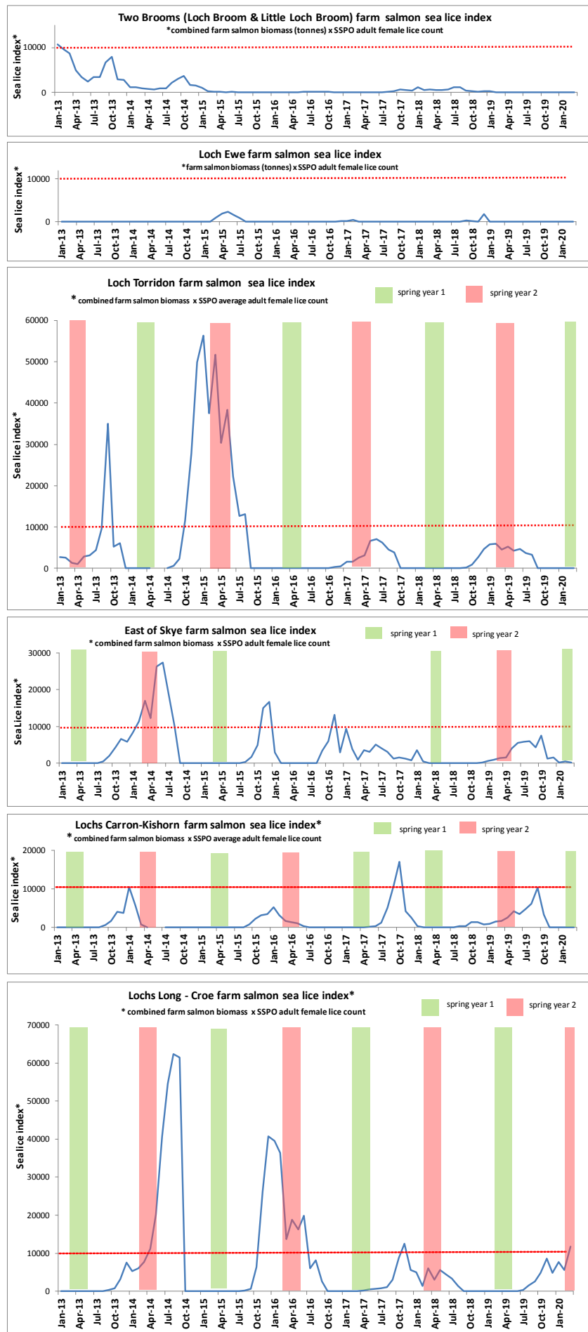
Figure 3.5. Sea lice indices for the east of the SWRFT area. See text above and Figure 3.6 for further explanation.
