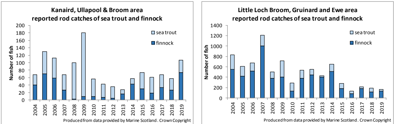
Figure 2.3 Rod catches of sea trout and finnock for north SWRFT mainland reporting areas.
