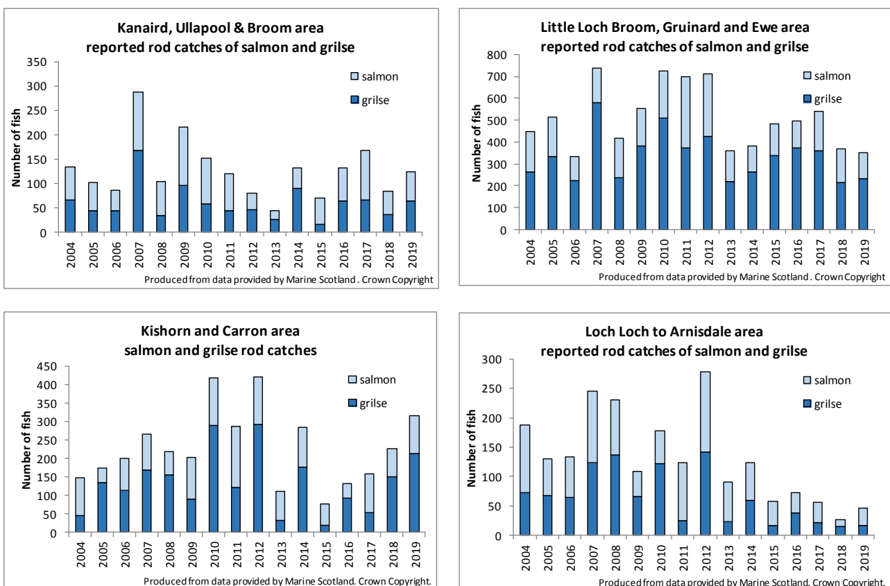
Figure 2.1 Rod catches of salmon and grilse for mainland parts of the SWRFT area.
