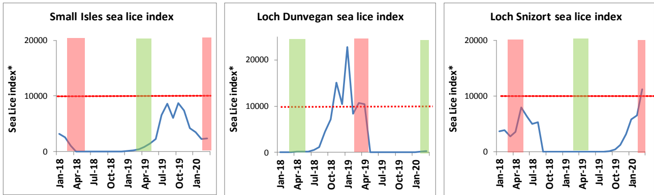
Figure 3.6. Sea lice indices for salmon farm production areas in the north and west of Skye.
