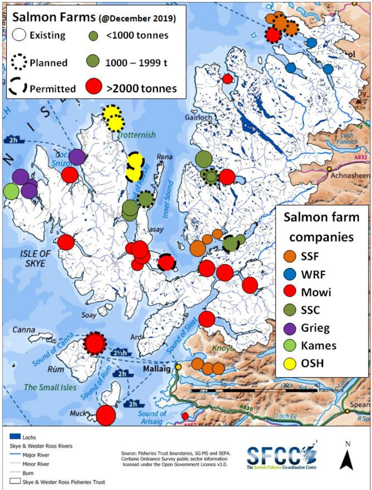
Figure 3.4. The Skye and Wester Ross Fisheries Trust area showing the locations of existing, planned and permitted new salmon farms within the area (as at December 2019).
