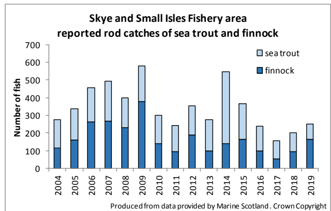
(right) Figure 2.5 Rod catches of sea trout for the Isle of Skye and Small Isles reporting area.
