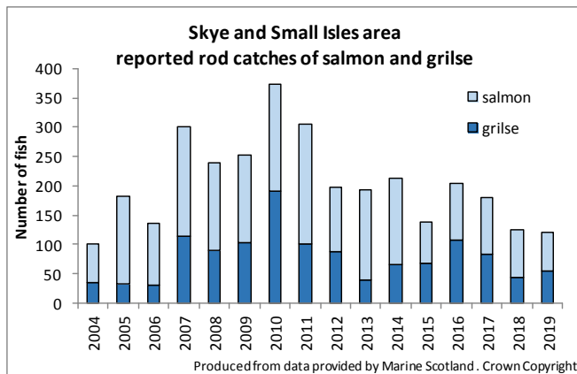
Figure 2.2 Rod catches of salmon and grilse for the Skye and Small Isles reporting area.
